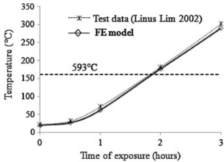
(a) Unexposed surface temperature
