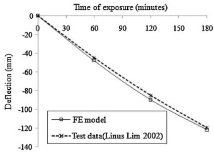
(b) Central deflection
